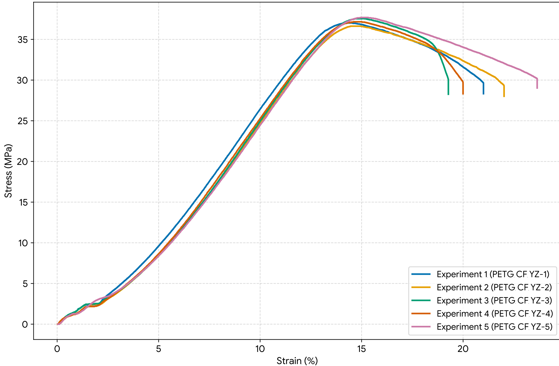
Stress-Strain Curves for PETG CF YZ (5 Experiments)
